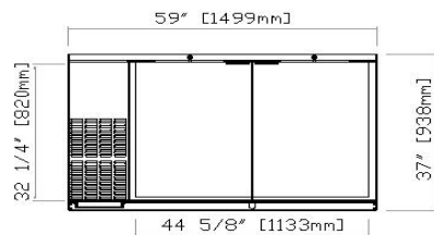
EBB(G) 58 FRONT
