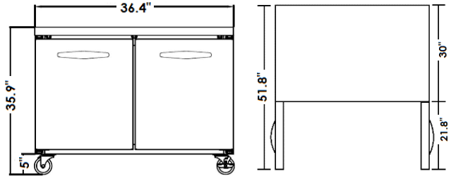
External Dimensions 36.4 x 30 x 35.9 (W" x D" x H") Internal Dimensions 32.4 x 26 x 27 (W" x D" x H")
