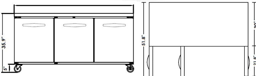
External Dimensions 72.4 x 30 x 35.9 (W" x D" x H") Internal Dimensions 68.4 x 26 x 27 (W" x D" x H")
