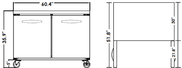
External Dimensions 60.4 x 30 x 35.9 (W" x D" x H") Internal Dimensions 56.4 x 26 x 27 (W" x D" x H")
