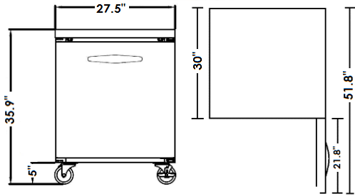
External Dimensions 27.5 x 30 x 35.9 (W" x D" x H") Internal Dimensions 23.5 x 26 x 27 (W" x D" x H")
