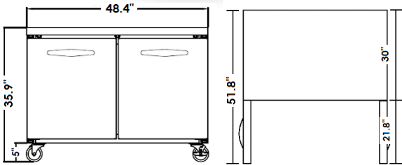
External Dimensions 48.4 x 30 x 35.9 (W" x D" x H") Internal Dimensions 44.4 x 26 x 27 (W" x D" x H")
